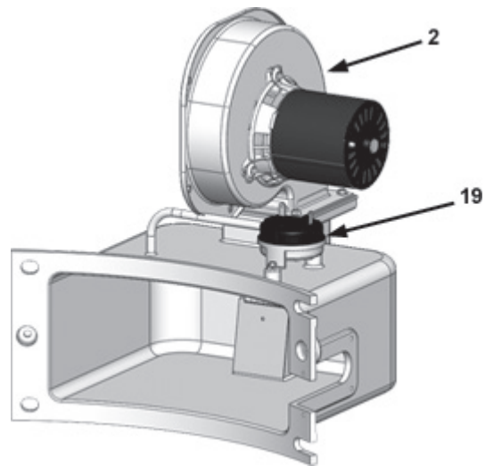
BLOWER ASSEMBLY
